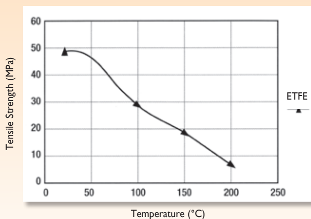
Effect of Temperature on Tensile Strength
